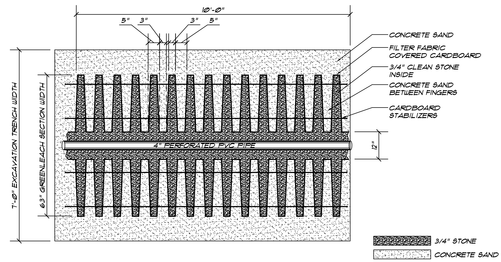
10' GREEN LEACH SYSTEM SECTION - TOP VIEW
