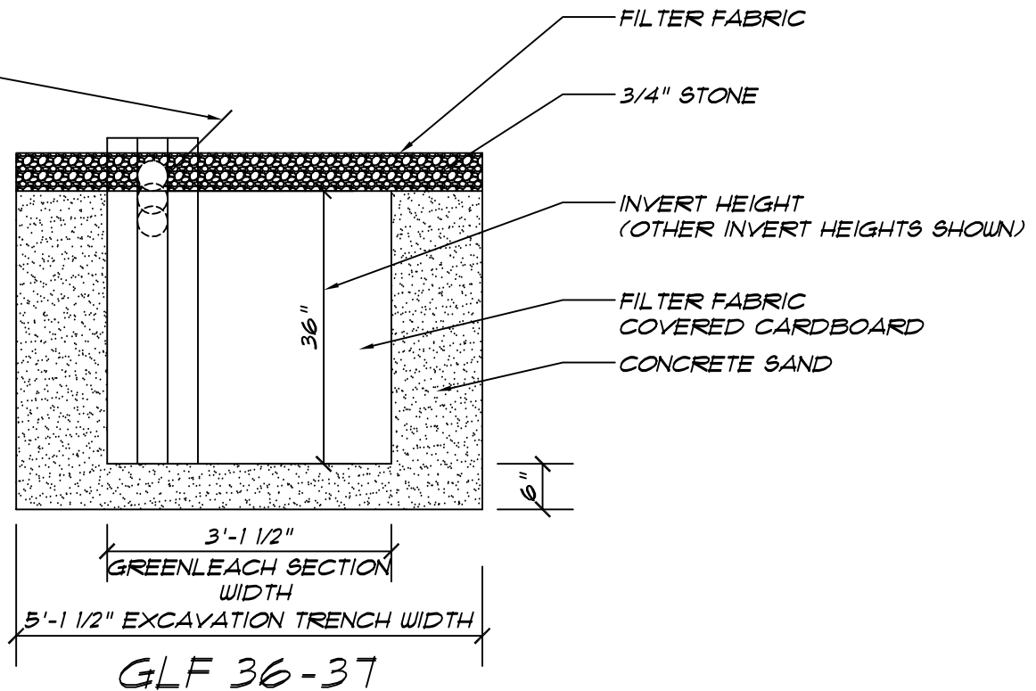
GREEN LEACH SYSTEM SECTION - END VIEW
